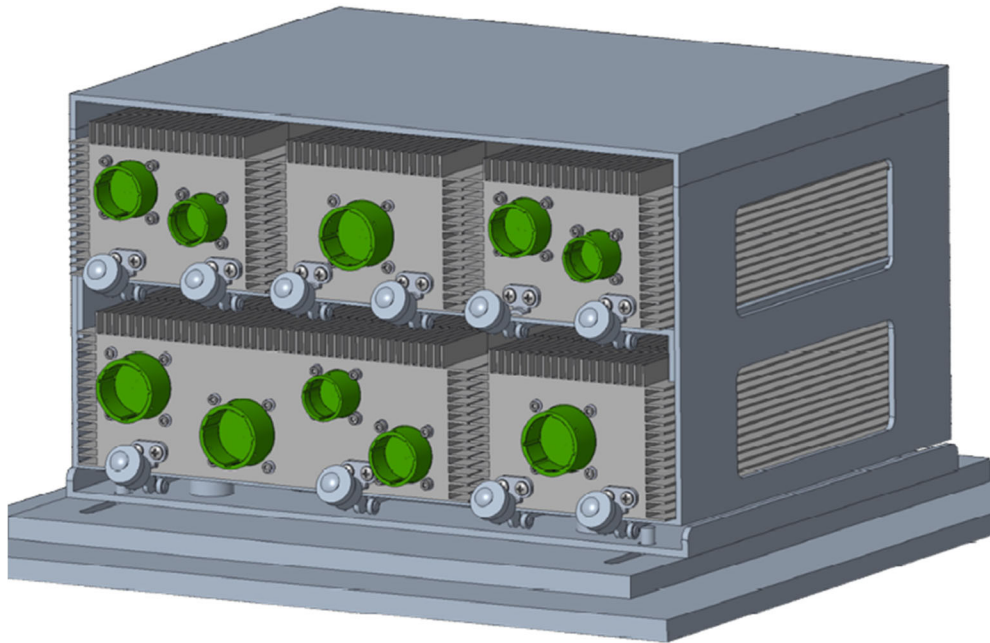
Figure 13. More efficient example of 5 devices sharing a single SAVE envelope
