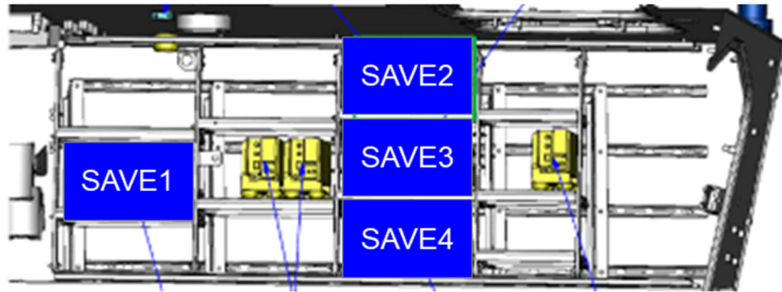
Figure 10. Notional platform with 4 SAVE envelopes - e.g. for Command or Retrans
