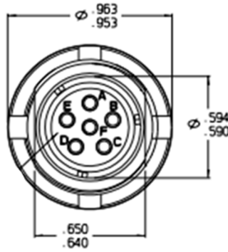
Figure 5. MIL-DTL-55116 Front Radio Audio Interface Connector
