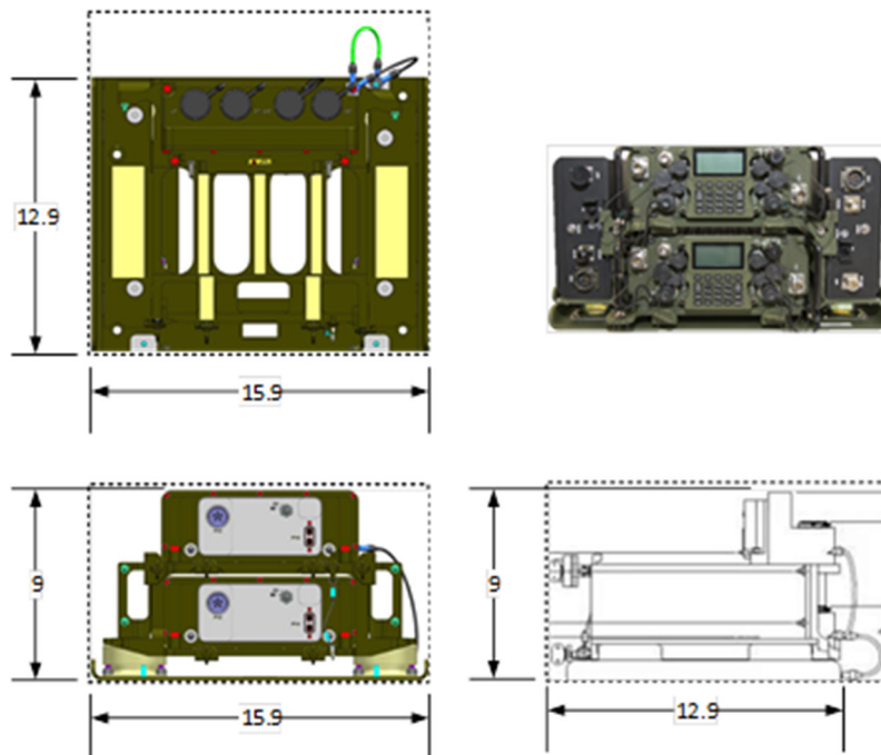
Figure 9. Collins Aerospace Dual HMS MP is SAVE compliant
