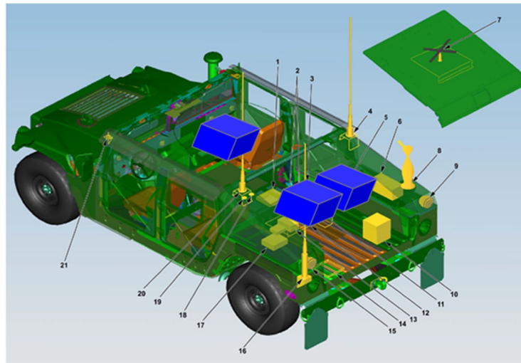
Figure 11. Notional platform with 3 SAVE envelopes
