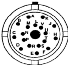
Figure 4. Rear M-1151 Vehicle Mount Audio Interface Connector
