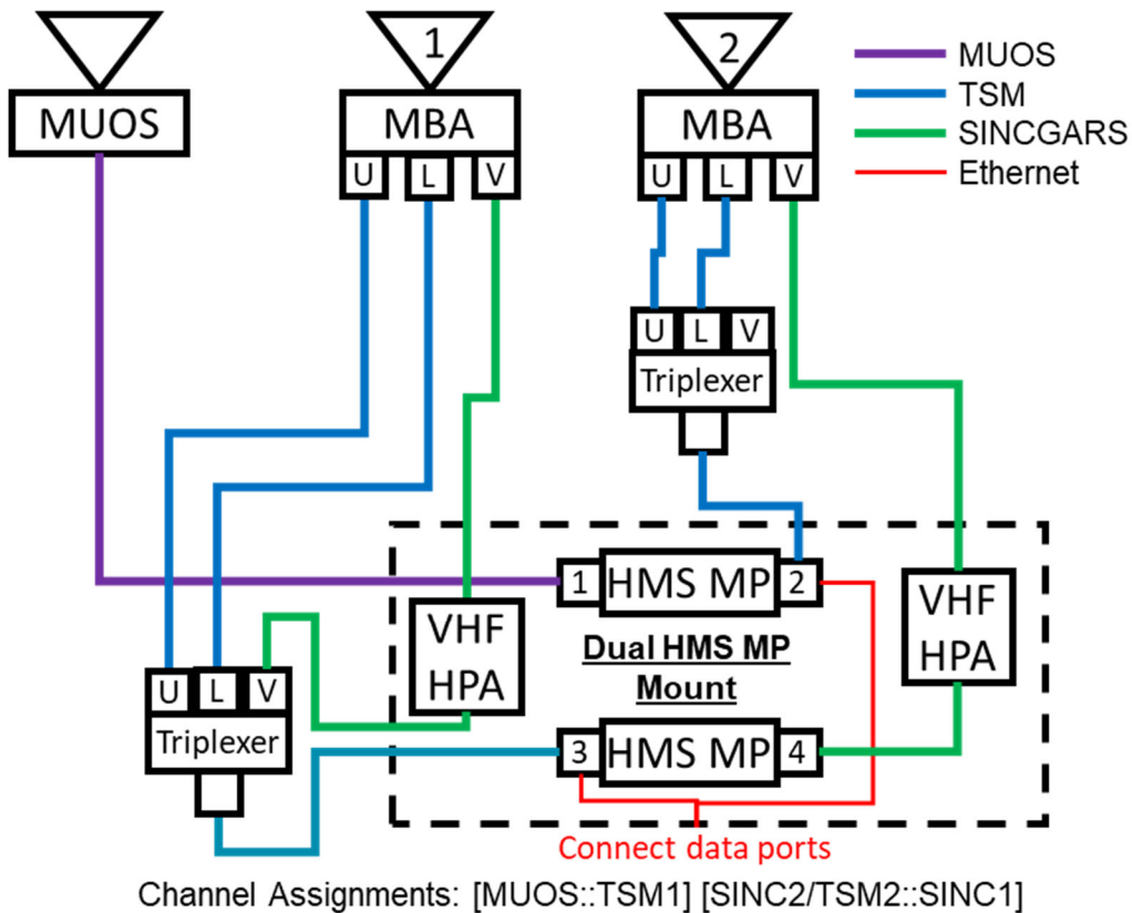
Figure 2. Example wiring for a Dual HMS MP with 2 MBAs
