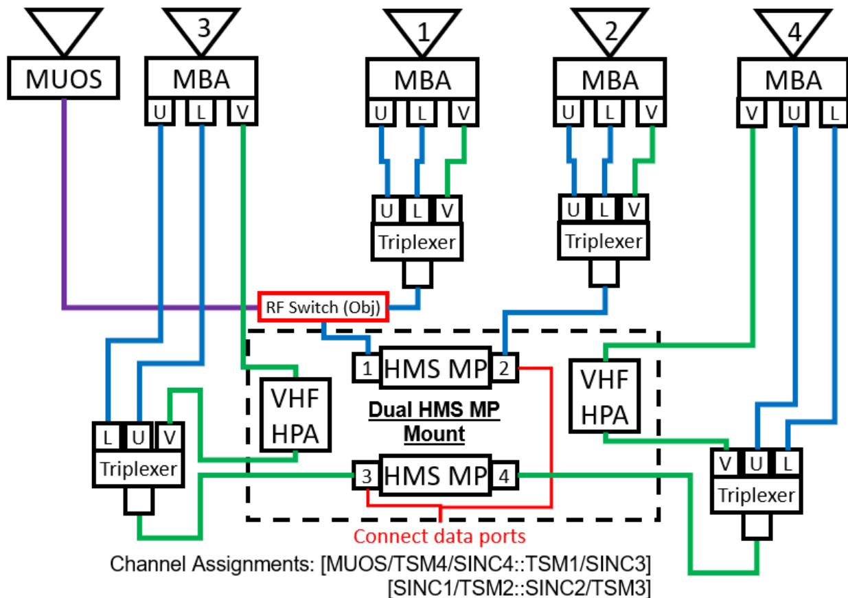
Figure 3. Example wiring for a Dual HMS MP with 4 MBAs
