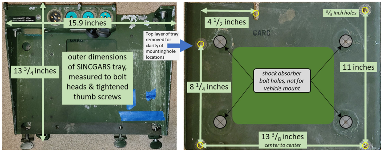
Figure 6. SINGGARS mounting hole pattern
