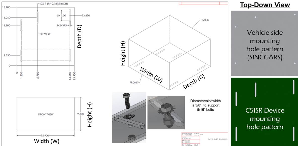
Figure 7. SAVE mounting hole pattern
