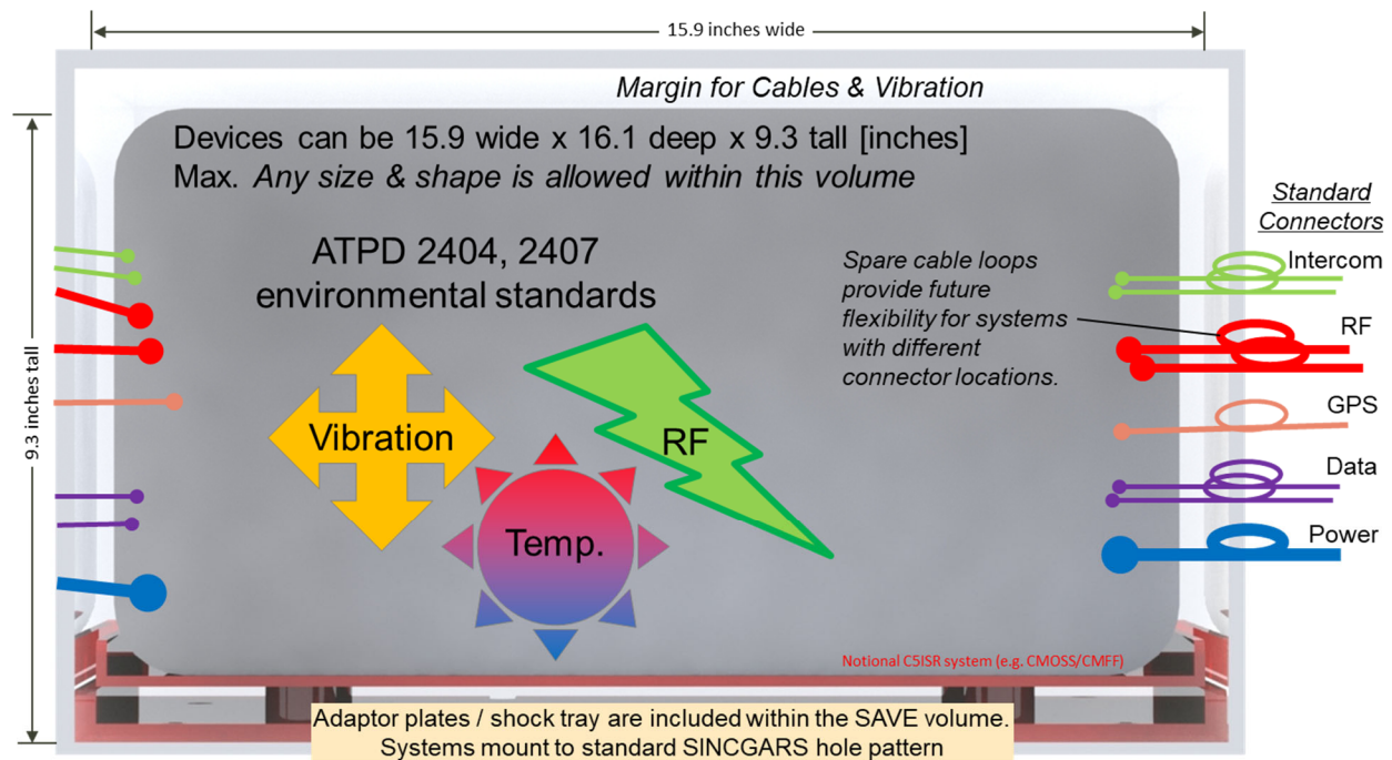
Figure 1. SAVE Envelope: Maximum Volume Allowed for SAVE Compliant Systems, Minimum Volume Provided by SAVE Compliant Vehicles
